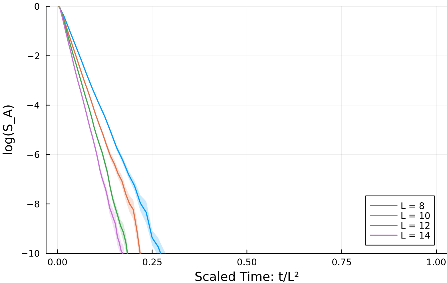
Scaled Log Entropy Evolution ( p = 0.666667 )
